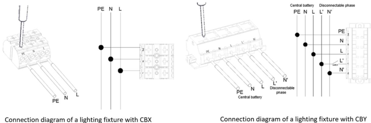
Figure 4. Possible connection diagrams of OptiLine **-*****CBX/CBY
